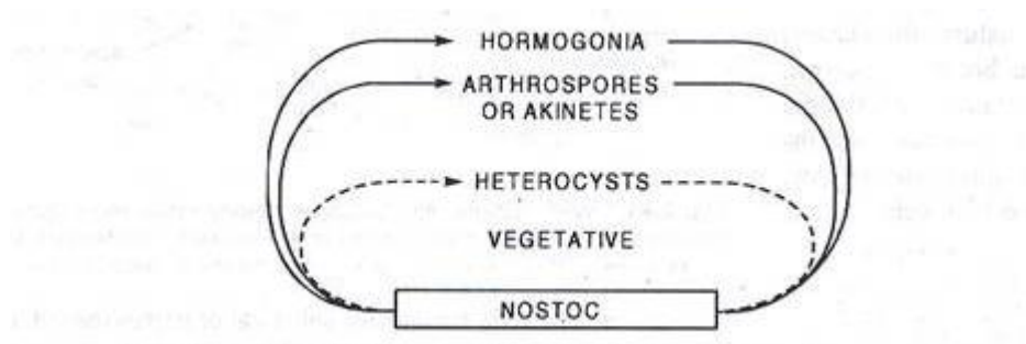
Figure 14- Cycle de vie de Nostoc
