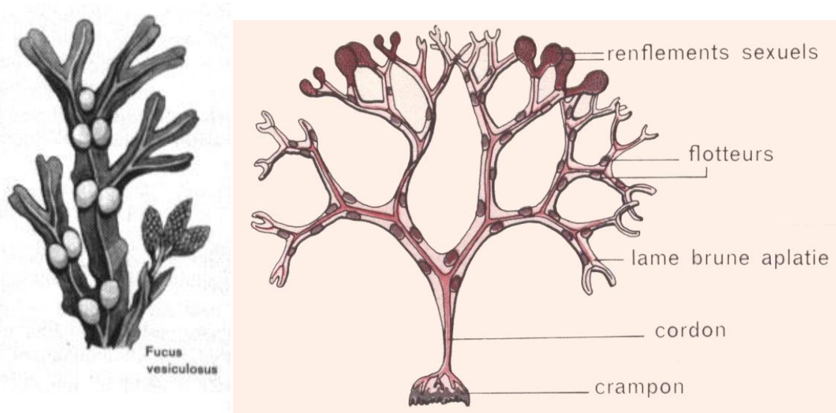
Figure 8- Aspect du thalle de Fucus vesiculosus
